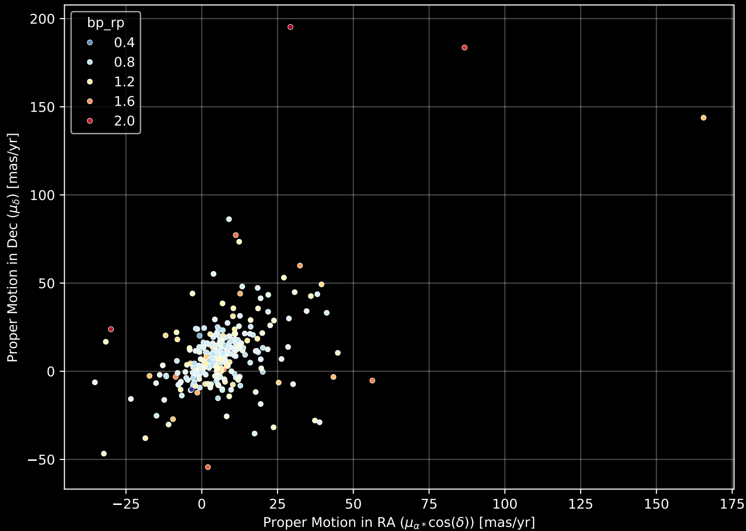
GALAH DR4 Field: [355] Proper Motion Diagram (n= 287)
