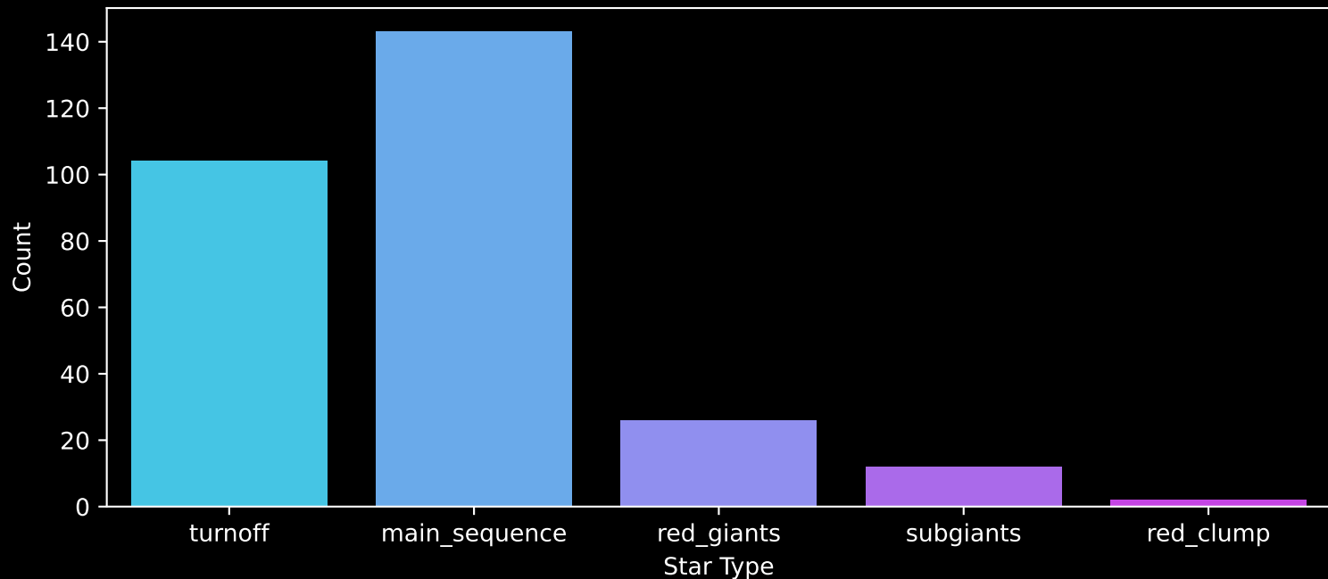
GALAH DR4 Field: [355] Count plot of Star Type
