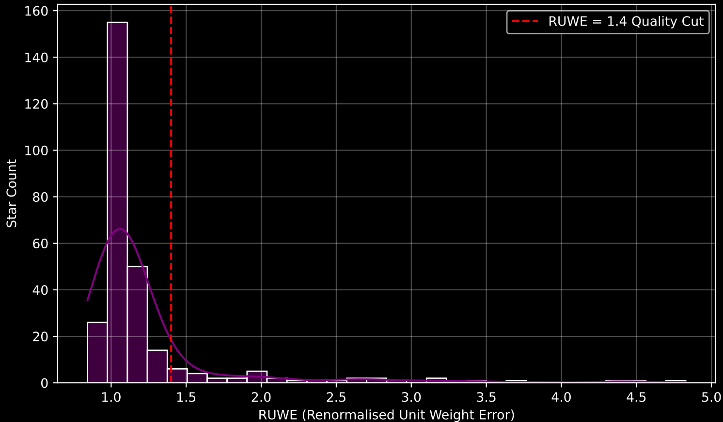
GALAH DR4 Field [355] RUWE Distribution (n= 281)
